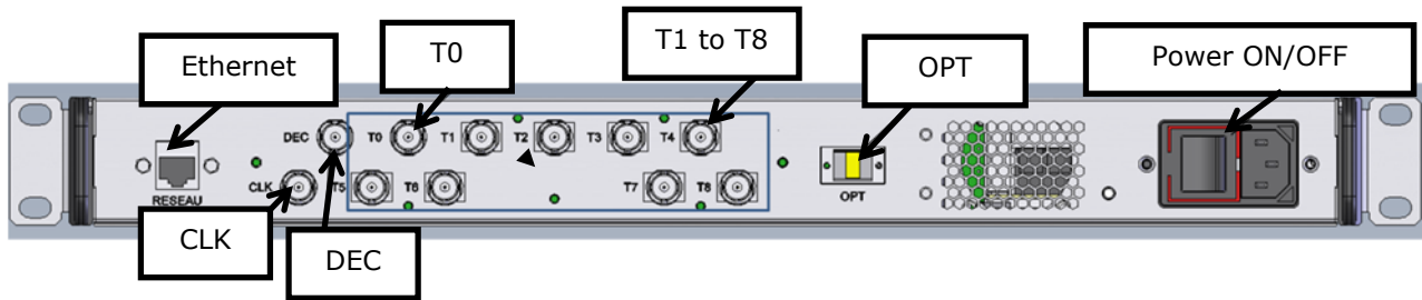
Rear panel
