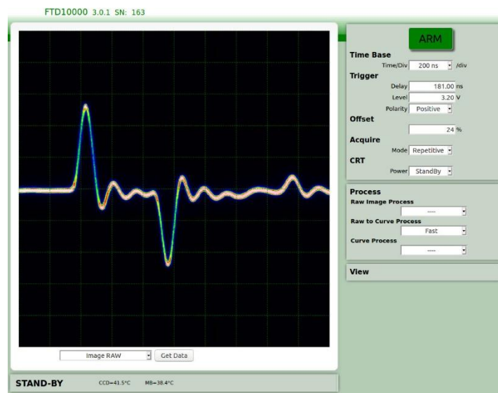
Remote GUI
