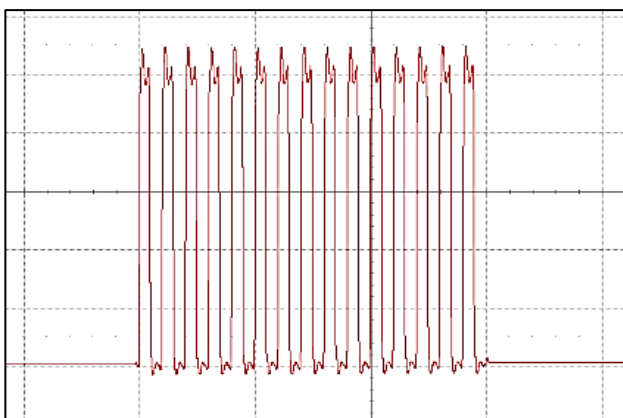
(100 ns/div, 2.0 V/div)
