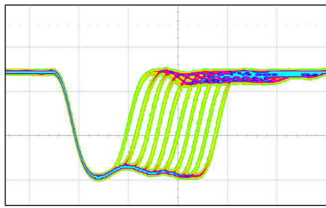
(500 ps/div, 0.5 V/div) View from scope in infinite persistence
