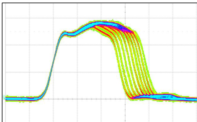
(1 ns/div, 2.0 V/div) View from scope in infinite persistence
