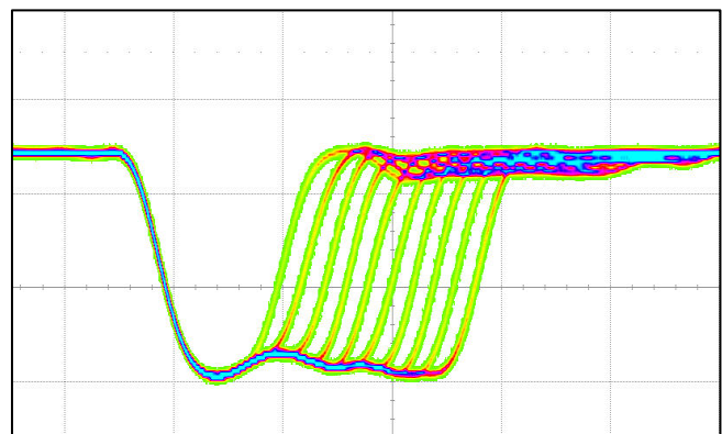
(500 ps/div, 0.5 V/div) View from scope in infinite persistence
