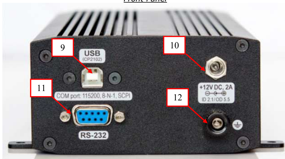
Rear Panel
